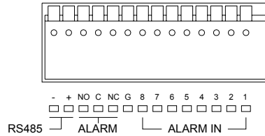
[Fig. 5-8 RS485 Connection]
